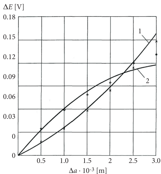
Fig. 3. The calculated curves and experimental values of difference EMF for various measurements of tubular products (× — experimental values of the signal with decrease in the thickness, ° — increase in the thickness)
