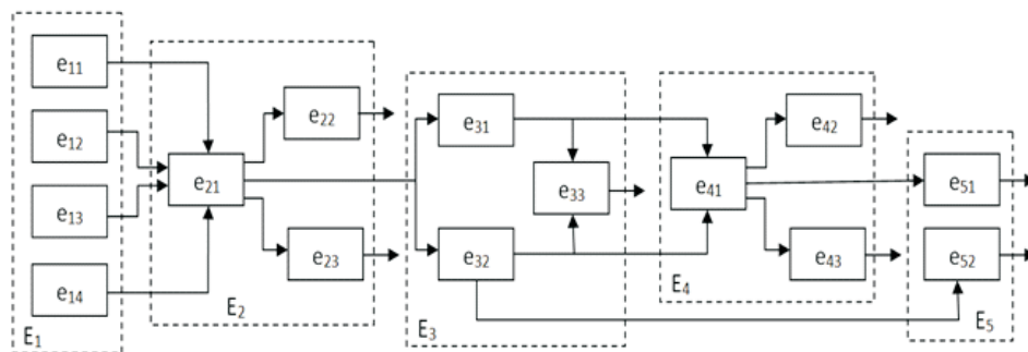
Fig. 3. Diagram of the functional and diagnostic structure of low-capacity solar power station equipment, with: E_1 — PV system; E_2 — voltage regulator system (controller module); E_3 — electrical power storage system; E_4 — DC/AC converter; E_5 — the load system
